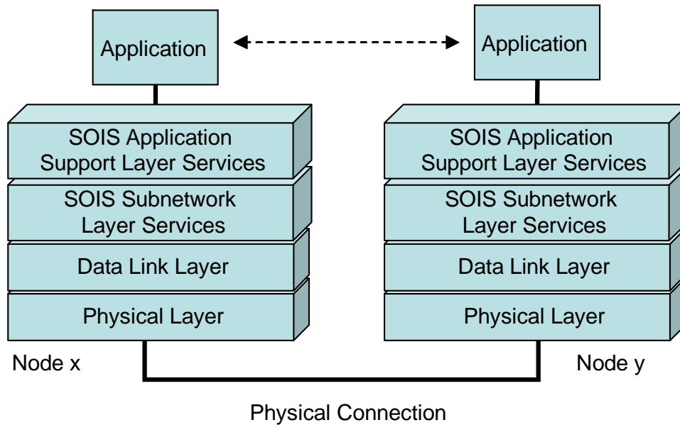
Figure 2-2: Symmetrical Communication
